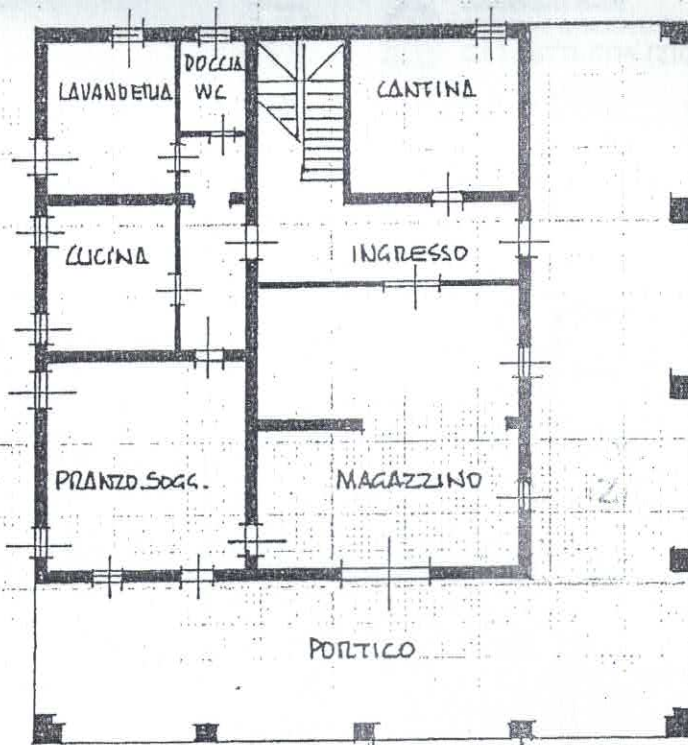
PIANO TERRA H 2.80
