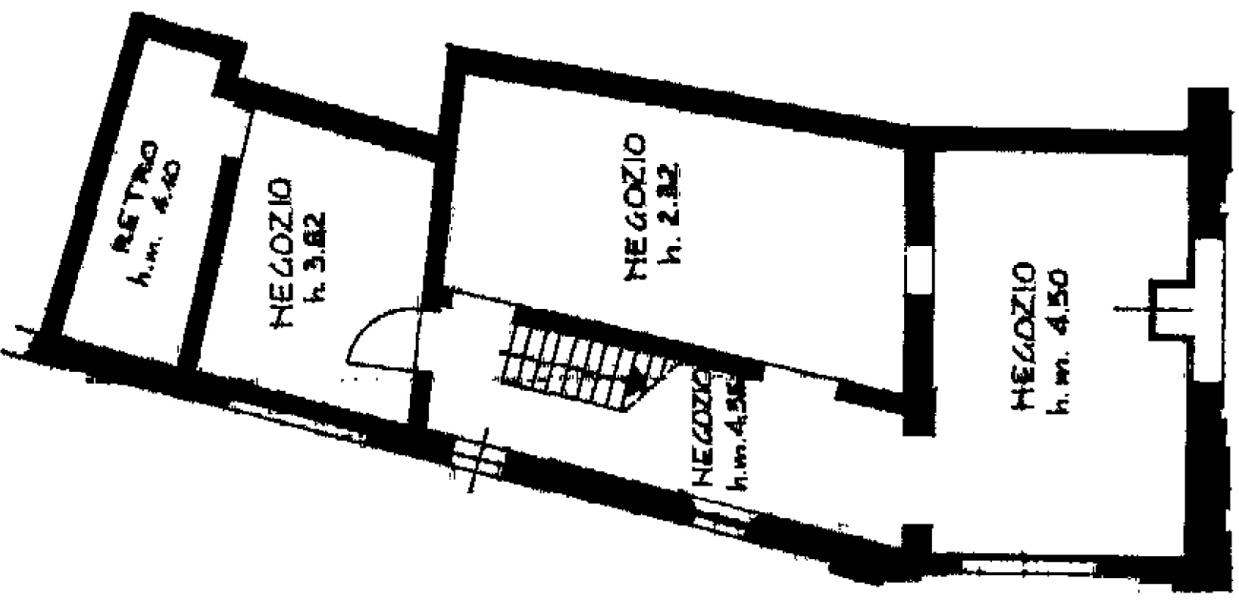
PIANO TERRA
