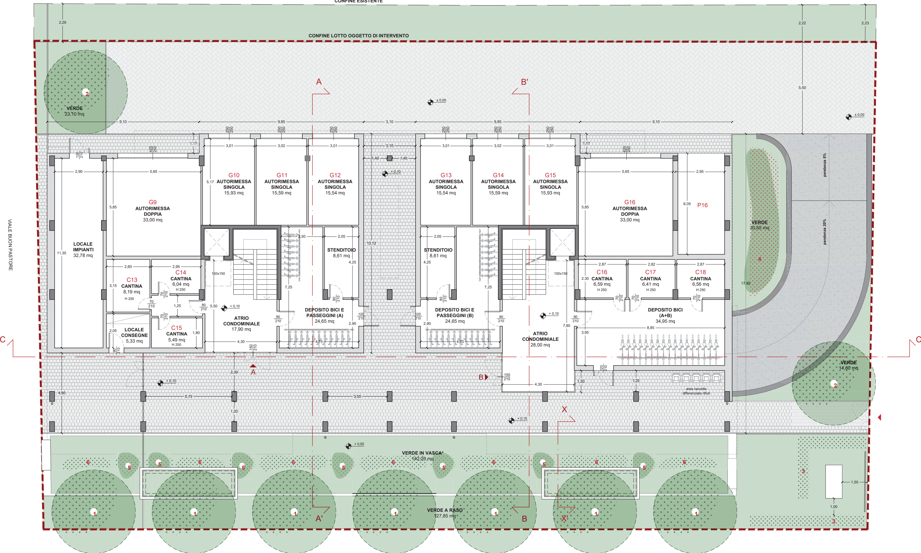
PIANO TERRA
